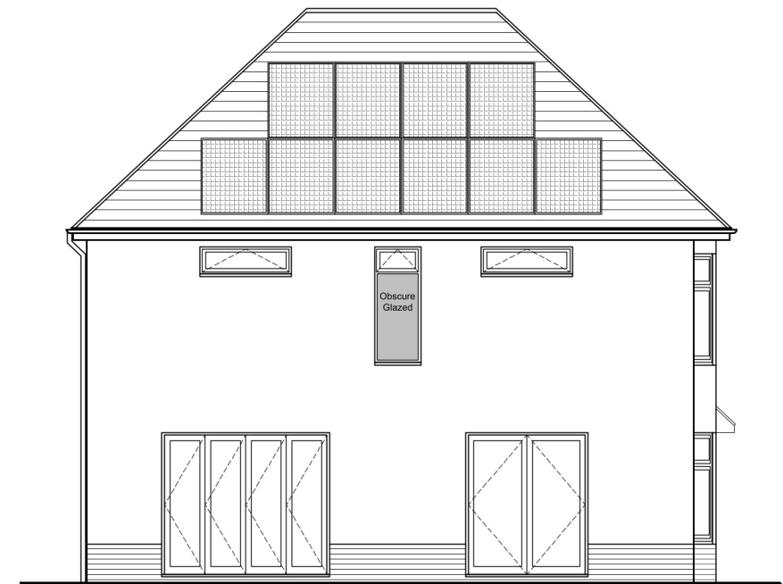
South East Elevation 1:100
