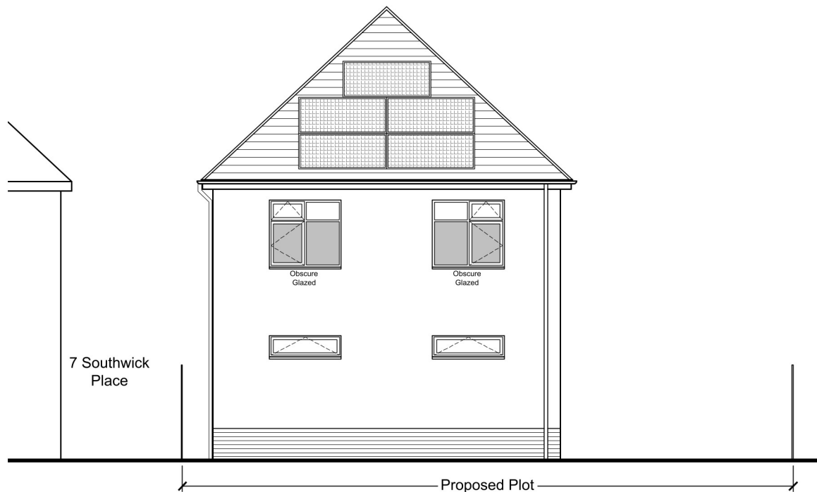
South West Elevation 1:100
