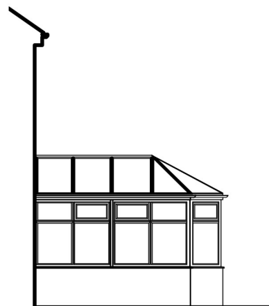
East (Sectional) Elevation 1:100
