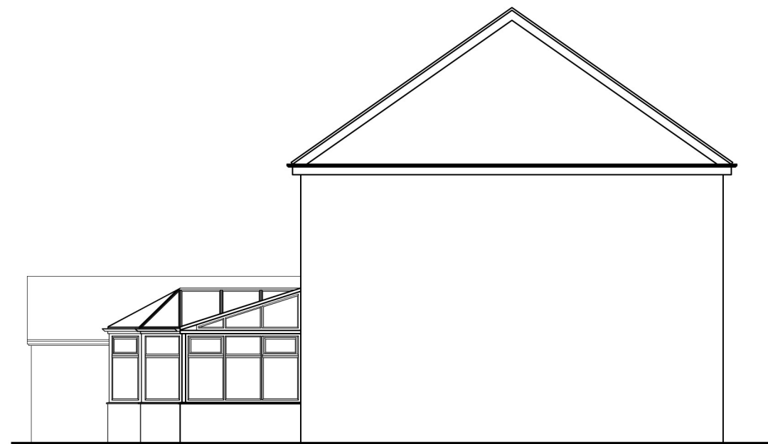
West Elevation 1:100
