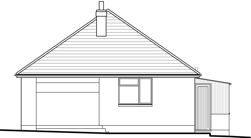
South Elevation 1:100
