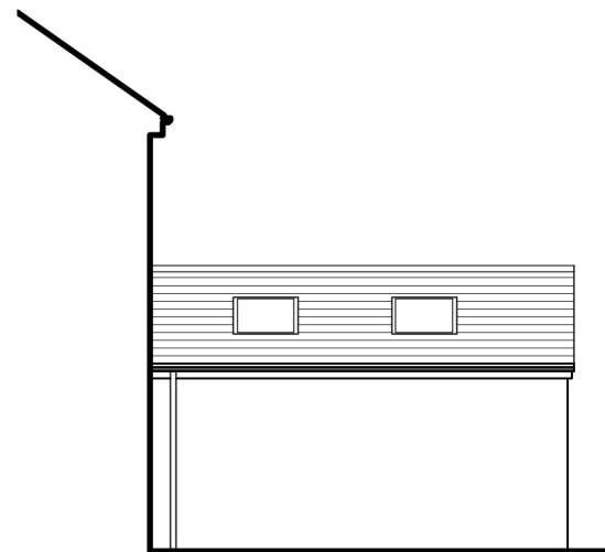
East (Sectional) Elevation 1:100
