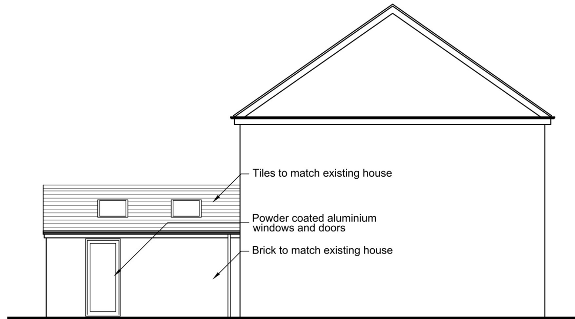
West Elevation 1:100
